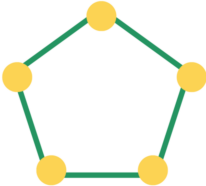
Pentagon(오각형)
