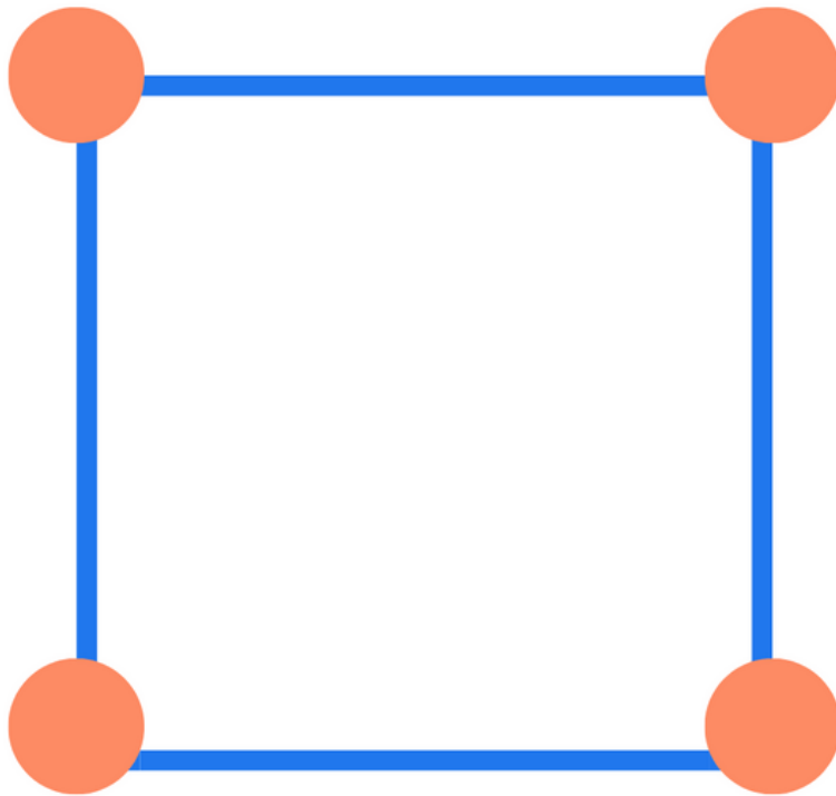
Square(정사각형)
