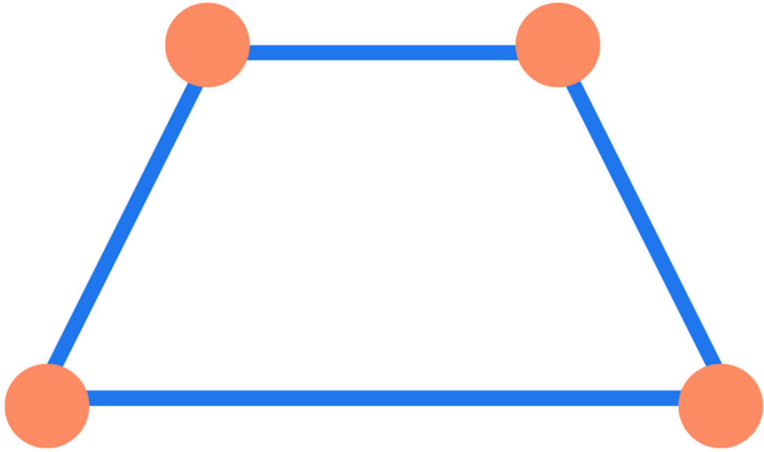
Trapezium (사다리꼴)
